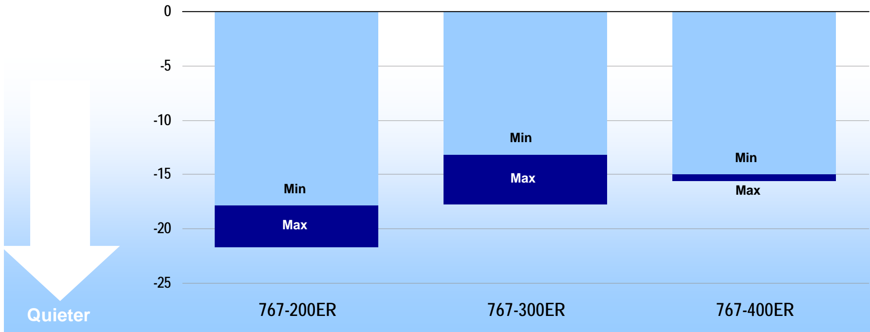
Cumulative margin below Stage 3, EPNdB
