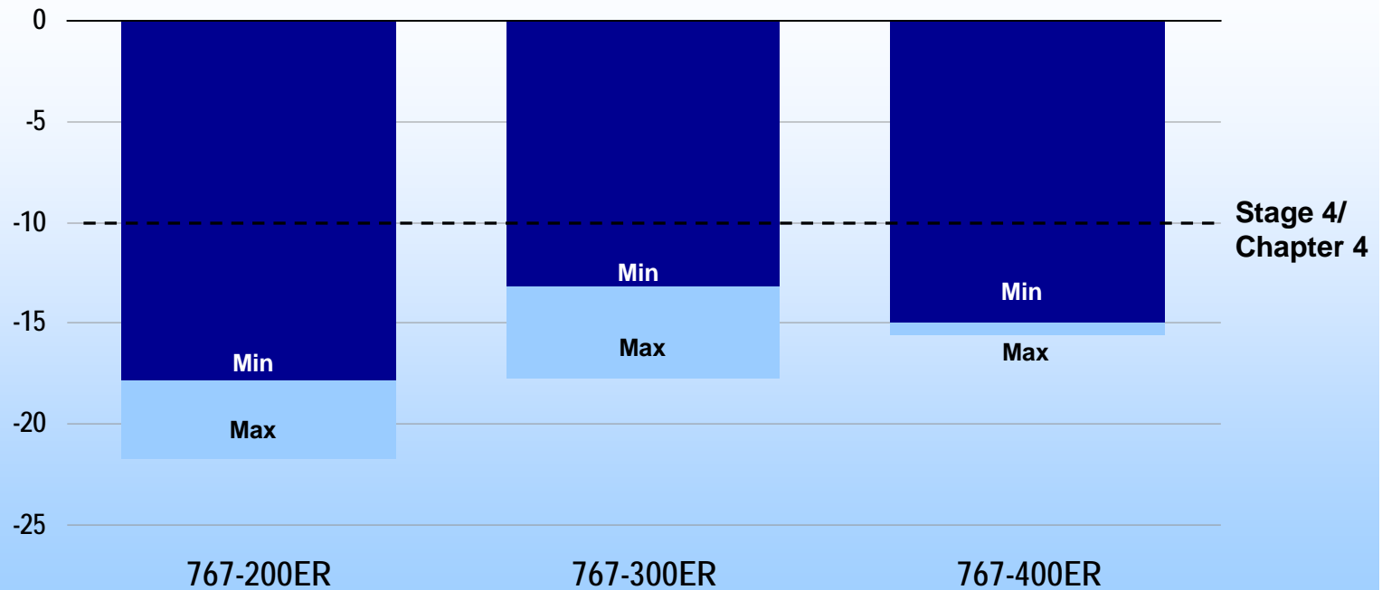
Cumulative margin below Stage 3, EPNdB
