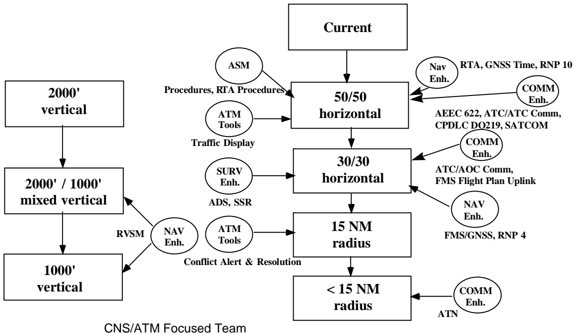
Figure 5.3: IATA Composite Transition Logic Diagram
