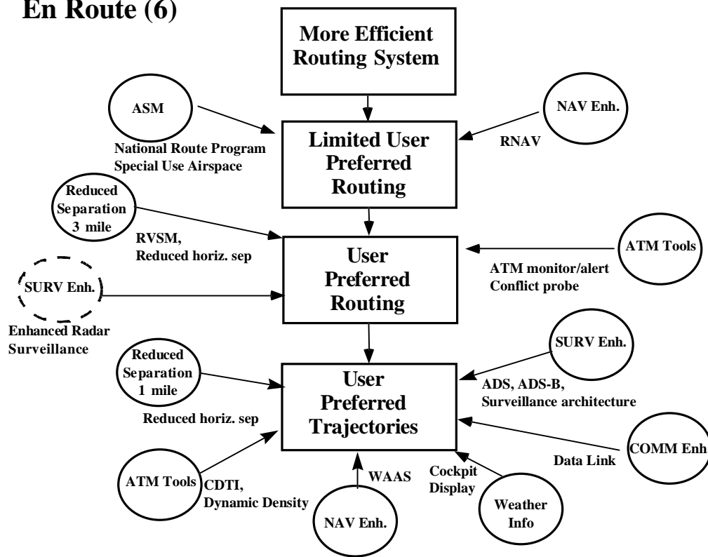
Figure 5.7: U.S. En Route Efficiency Transition Logic Diagram
