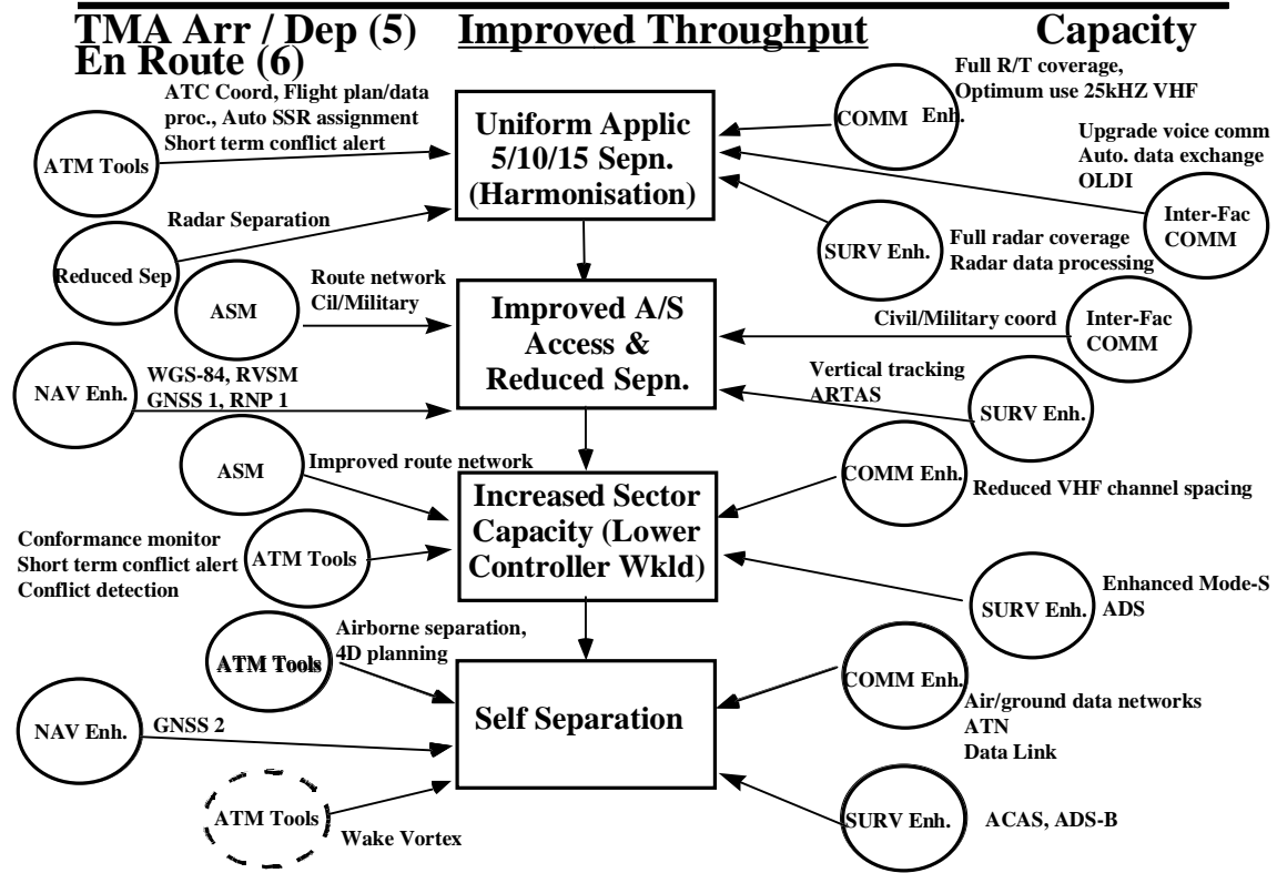
Figure 5.5: European En Route Capacity Transition Logic Diagram
