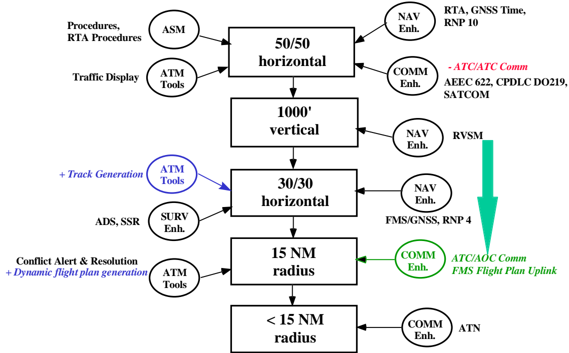
Figure 5.4: IATA Asia CAISC Transition Logic Diagram
