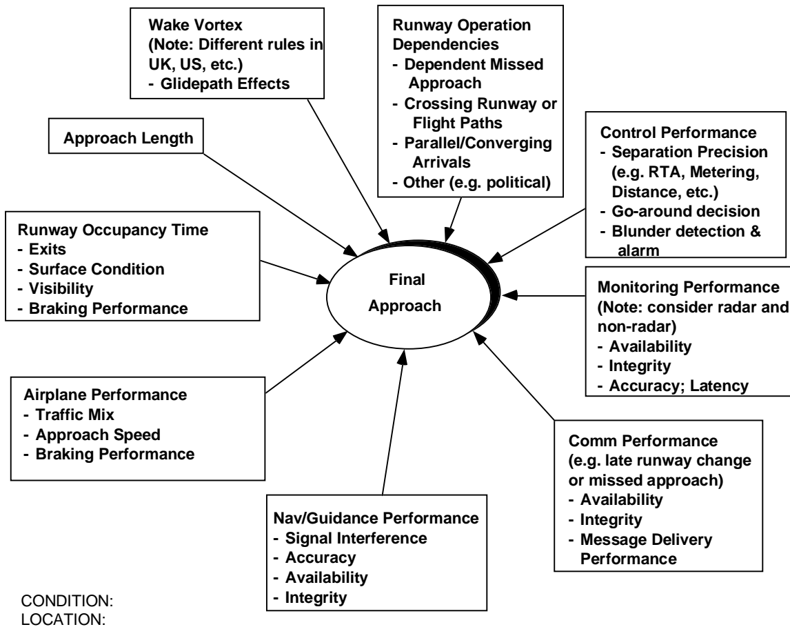
Figure 4.4: Throughput Performance Factors for Final Approach
