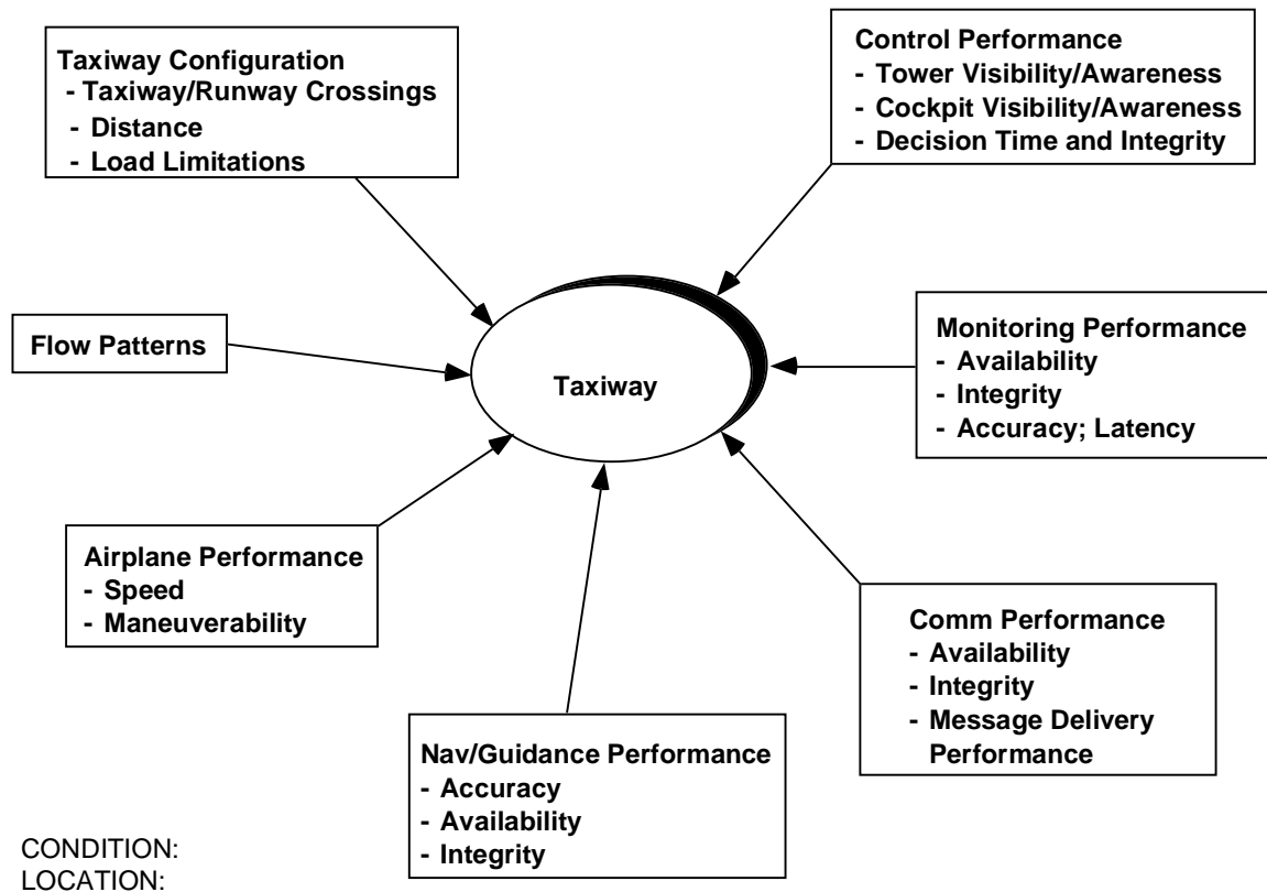
Figure 4.3: Taxiway Performance Factors
