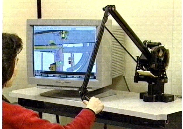
Figure 9. User with the 6-DOF haptic device.
