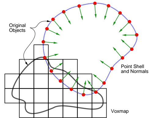
Figure 1. Voxmap colliding with point shell.
