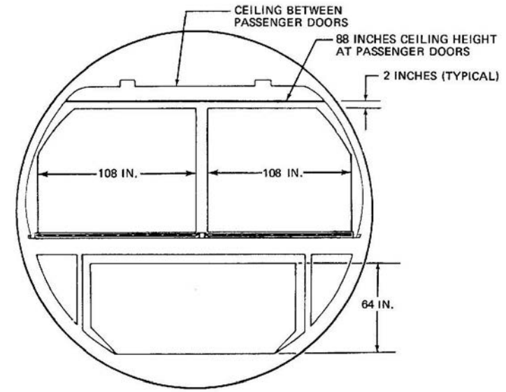
Convertible Freighter Configuration
