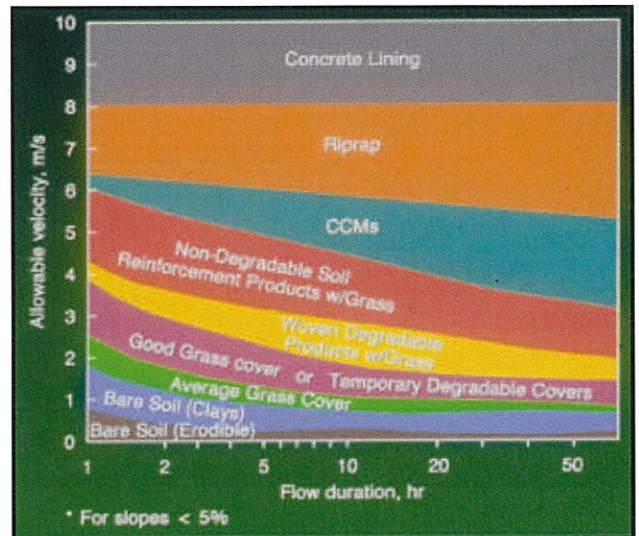
Figure 2. Erosion limits as a function of flow duration (from Fischenich and Allen (2000)).
