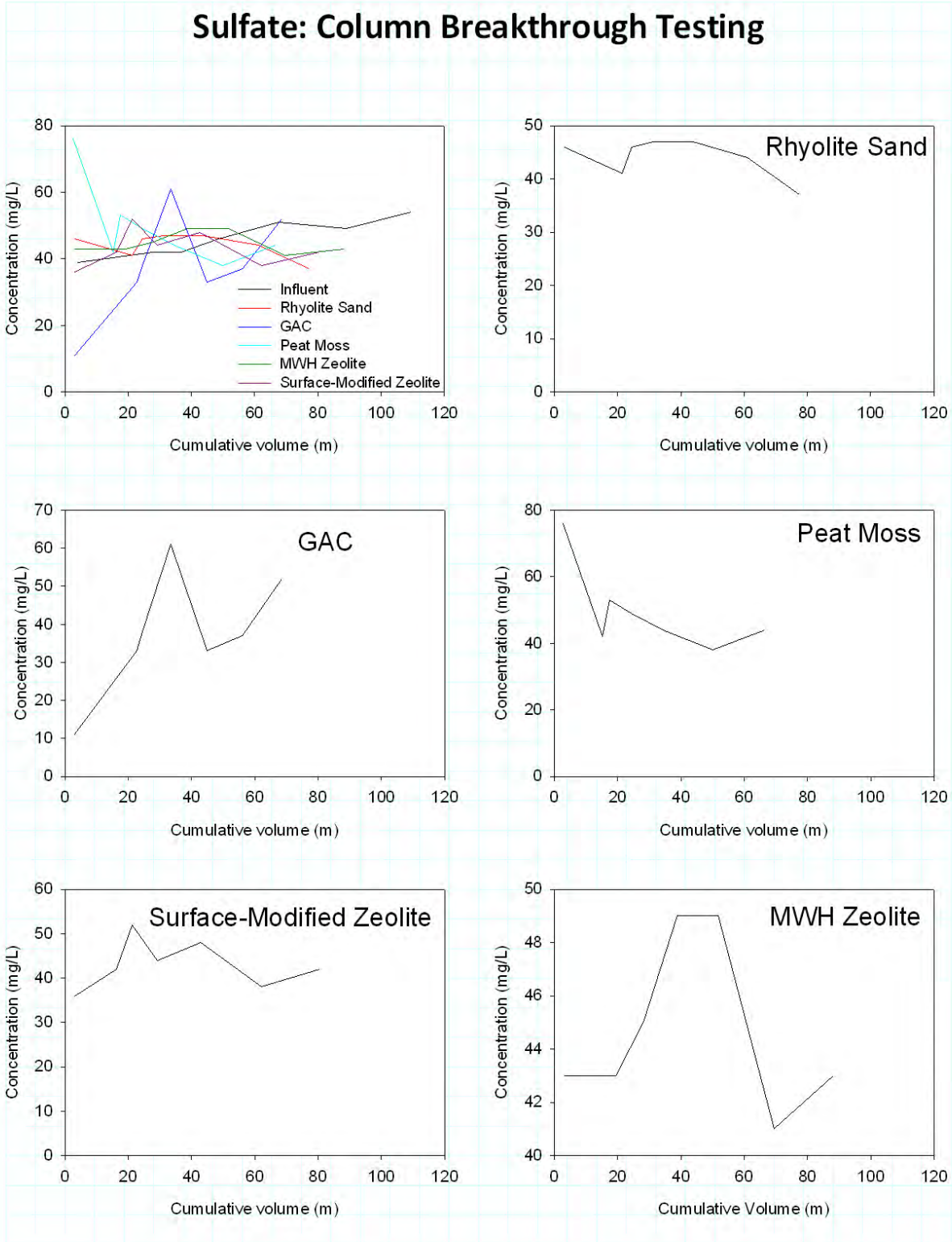
Figure A3-43. Breakthrough plots for sulfate.
