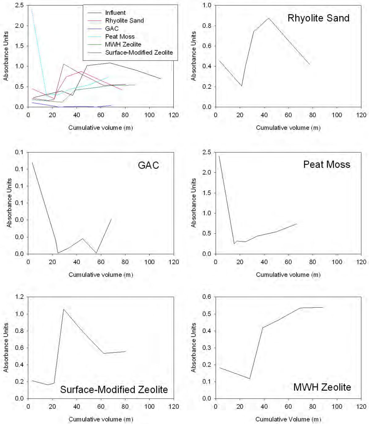
Figure A3-49. Breakthrough plots for UV-254.
