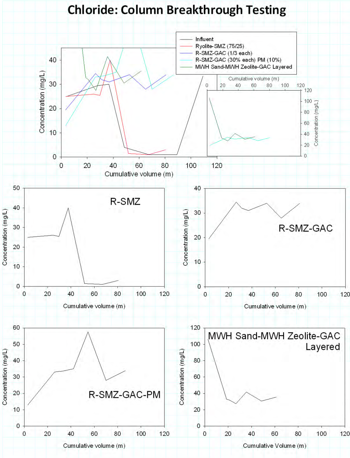
Figure A3-14. Breakthrough plots for chloride (cont.).
