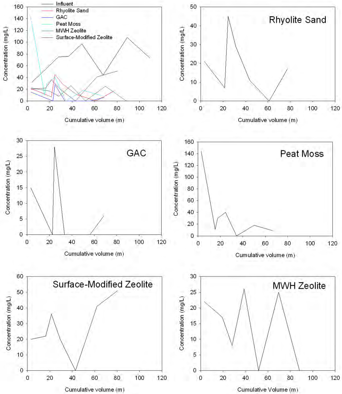
Figure A3-17. Breakthrough plots for COD.
