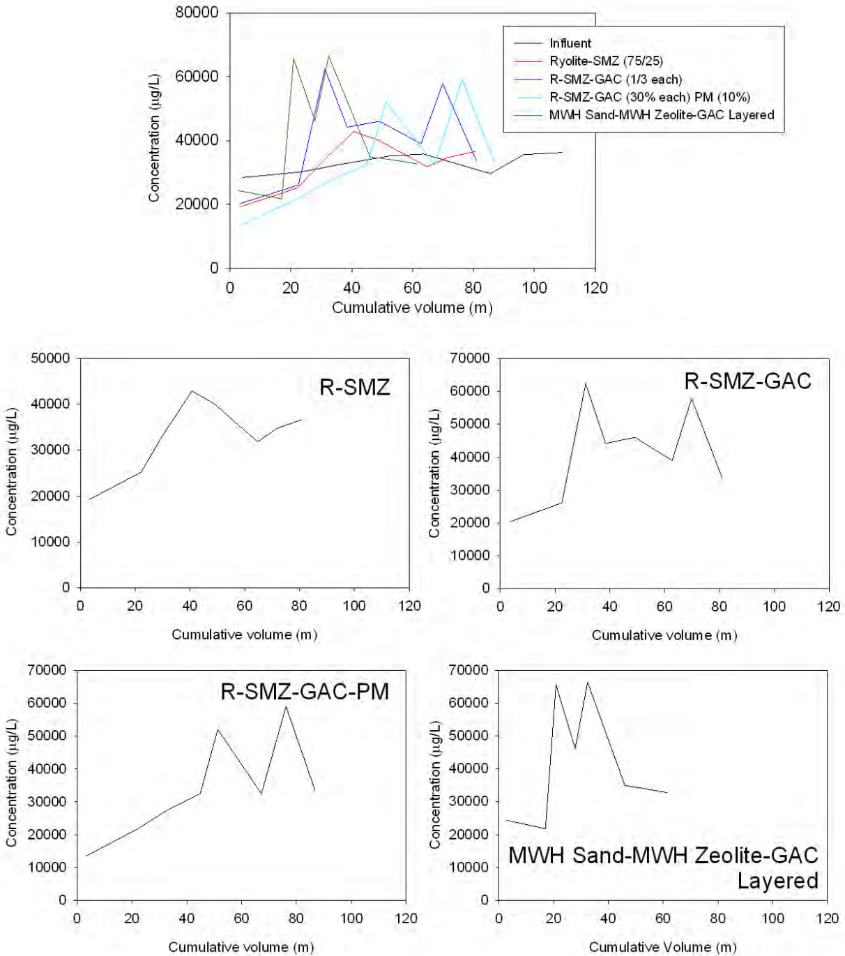
Figure A3-12. Breakthrough plots for total calcium (cont.).
