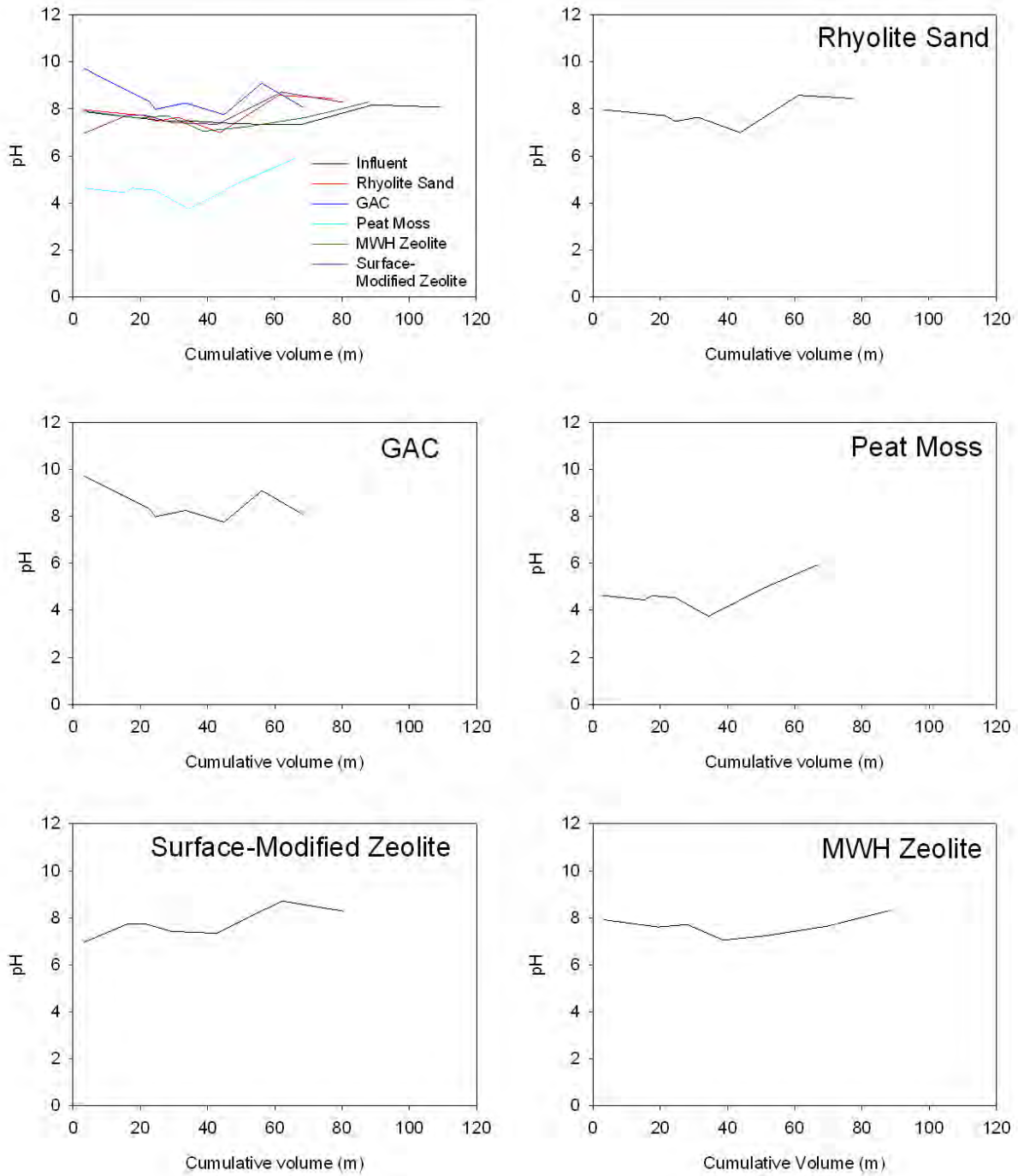
Figure A3-37. Breakthrough plots for pH.
