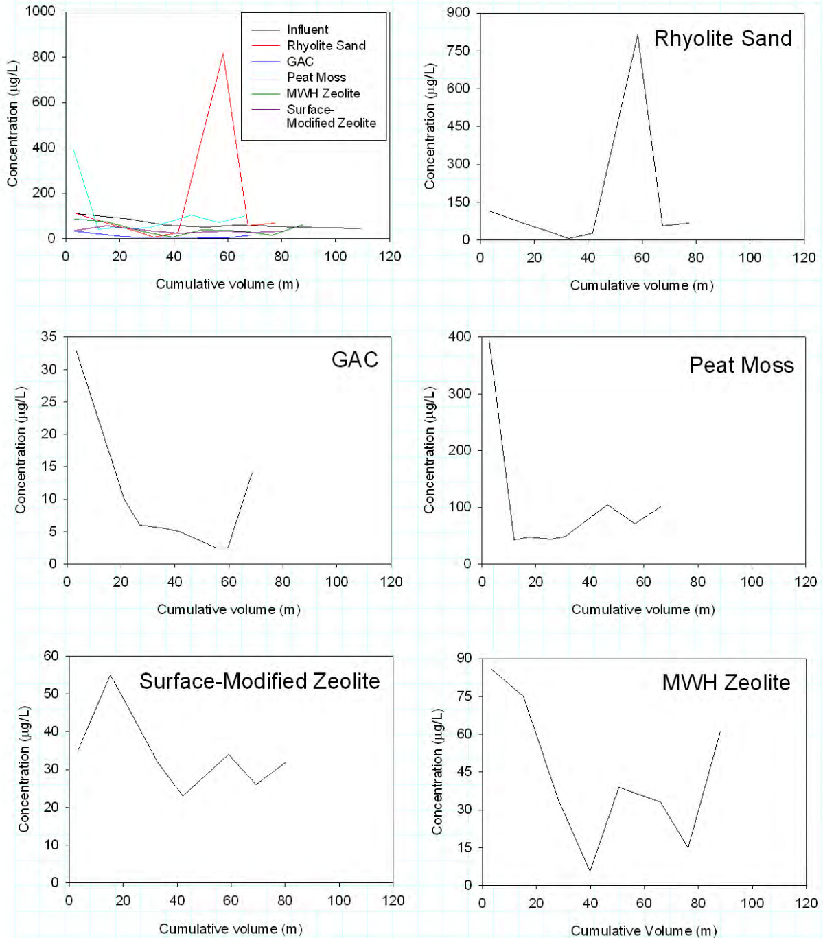
Figure A3-24. Breakthrough plots for filtered iron.
