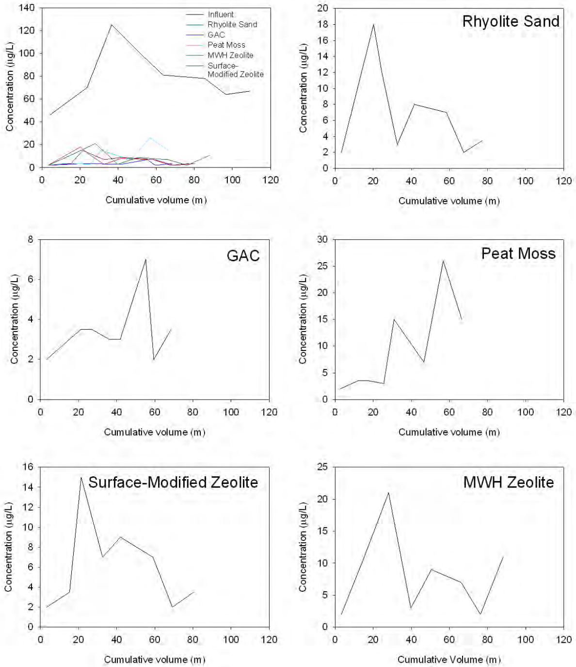
Figure A3-45. Breakthrough plots for total thallium.
