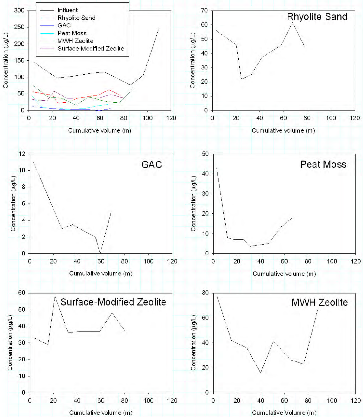
Figure A3-20. Breakthrough plots for total copper.
