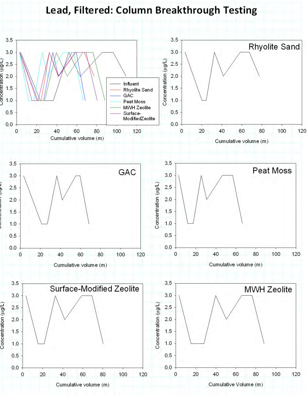
Figure A3-26. Breakthrough plots for filtered lead.
