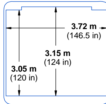
Main deck cargo door (STA 1713.75)
